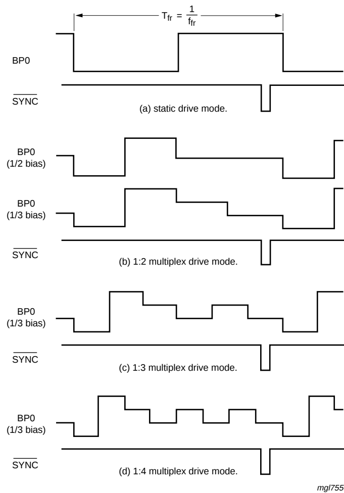
Fig 21. Synchronization of the cascade for the various PCF85133 drive modes
