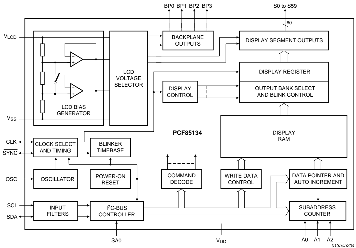
Fig 1. Block diagram of PCF85134
