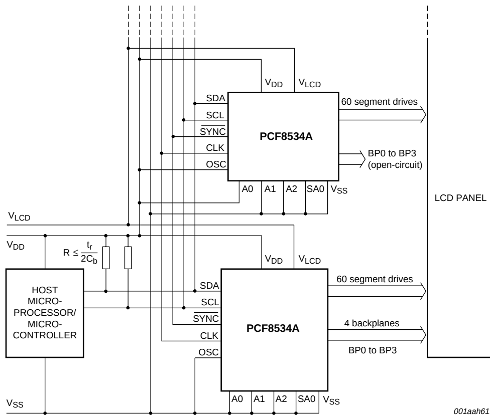
Fig 22. Cascaded PCF8534A configuration
