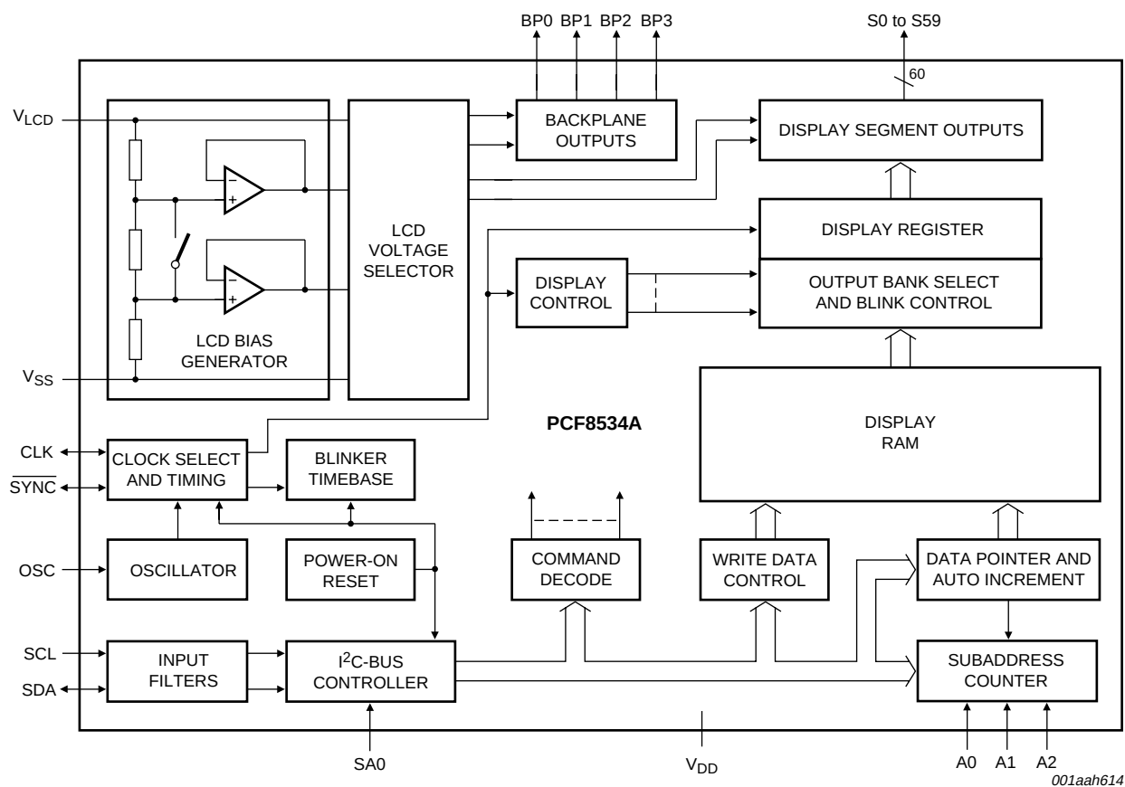
Fig 1. Block diagram of PCF8534A
