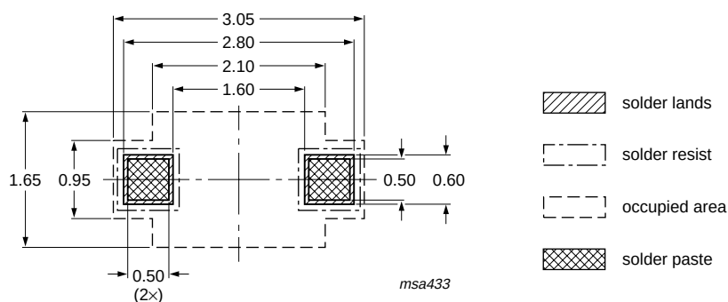
Fig 9. Reflow soldering footprint SOD323 (SC-76)
