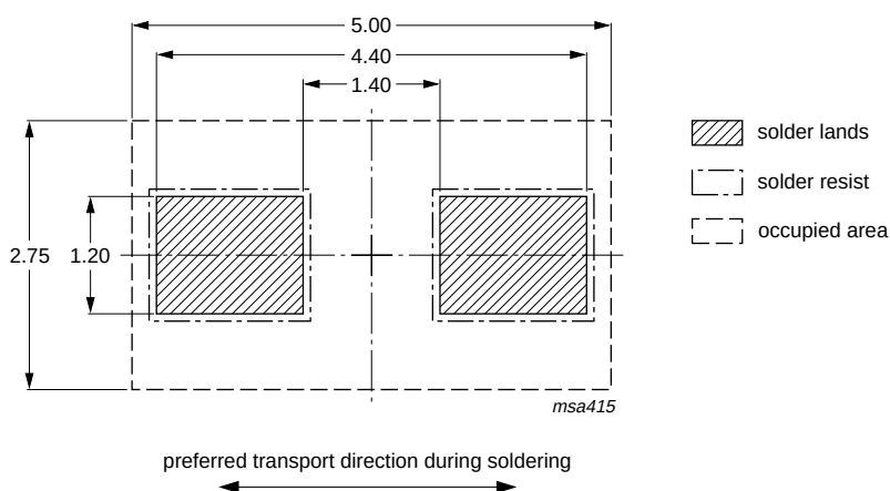
Fig 10. Wave soldering footprint SOD323 (SC-76)
