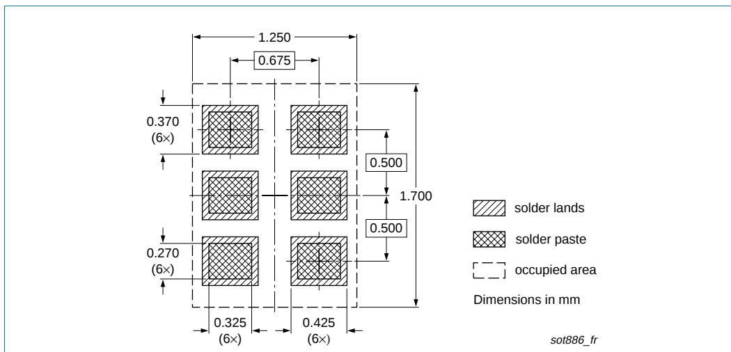
Fig 8. Reflow soldering footprint PESD5V0U4BF (SOT886)
