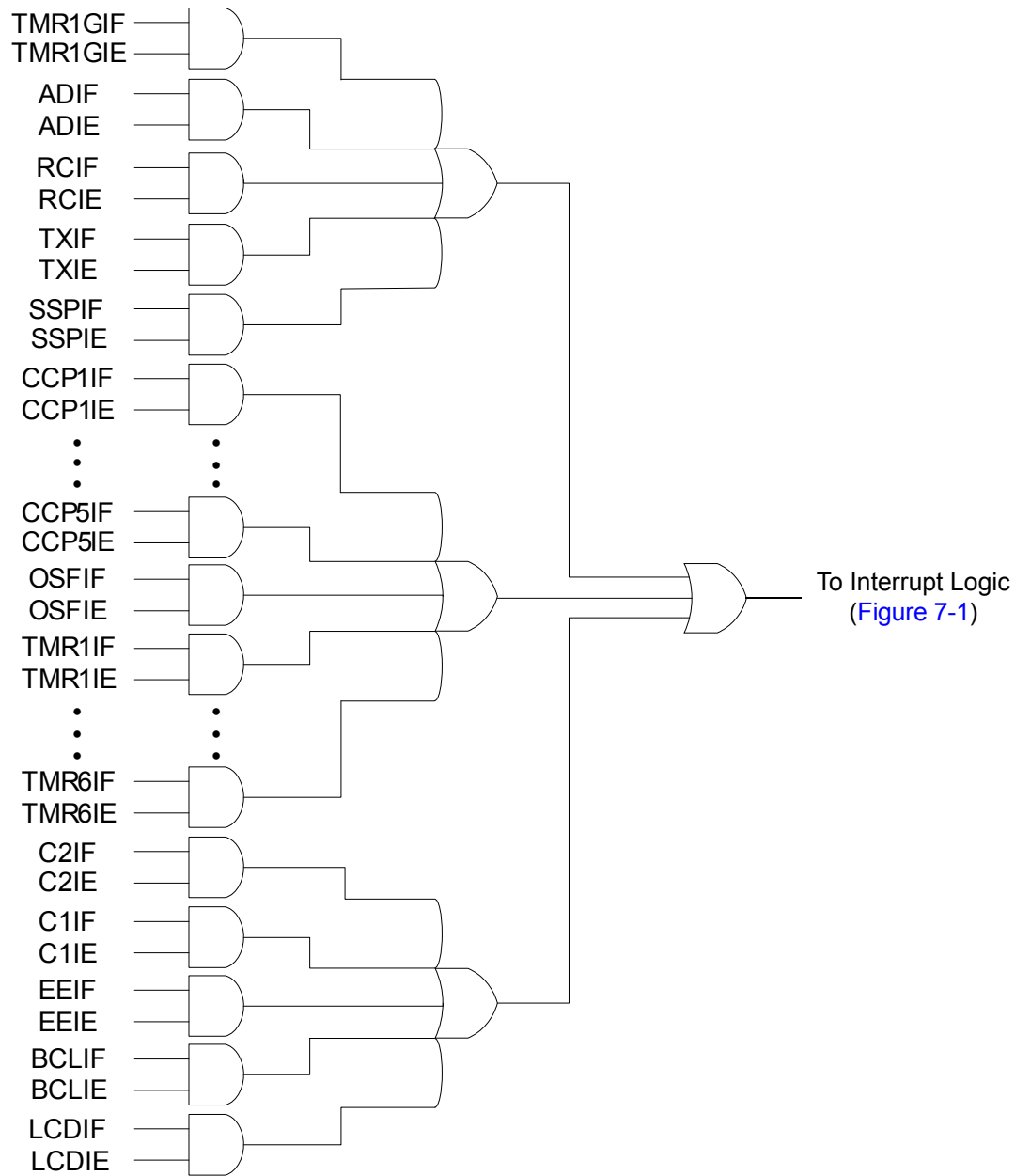
FIGURE 7-2: PERIPHERAL INTERRUPT LOGIC
