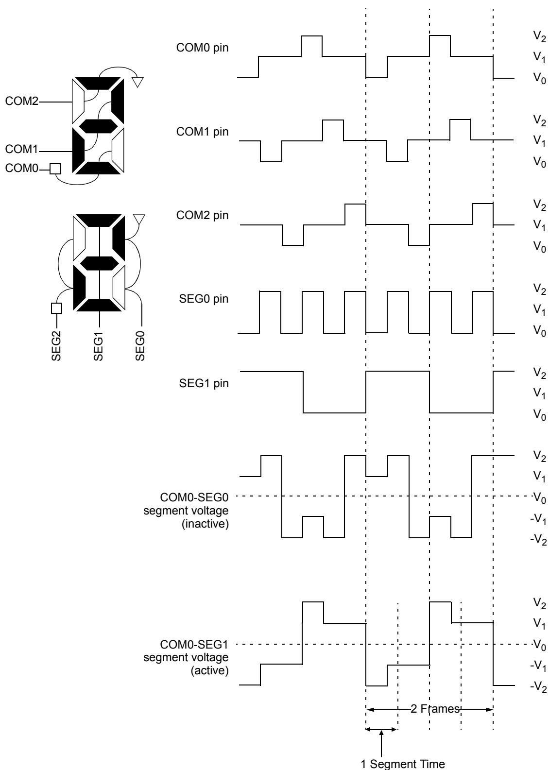
FIGURE 27-14: TYPE-B WAVEFORMS IN 1/3 MUX, 1/2 BIAS DRIVE
