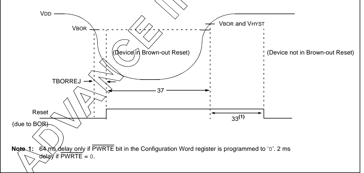
FIGURE 27-9: BROWN-OUT RESET TIMING AND CHARACTERISTICS
