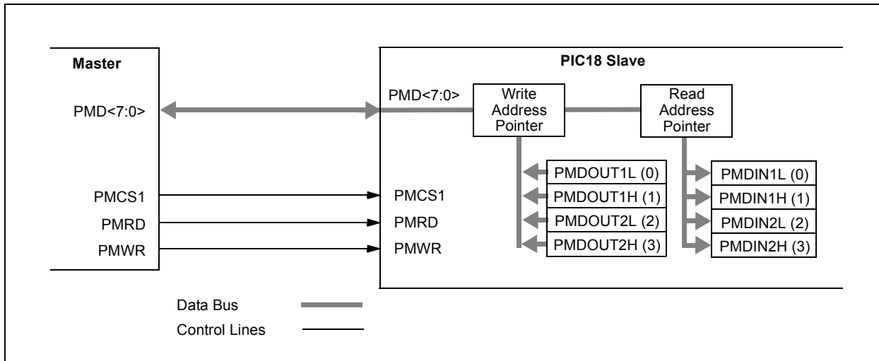
FIGURE 11-5: PARALLEL MASTER/S�AVE CONNECTION BUFFERED EXAMPLE
