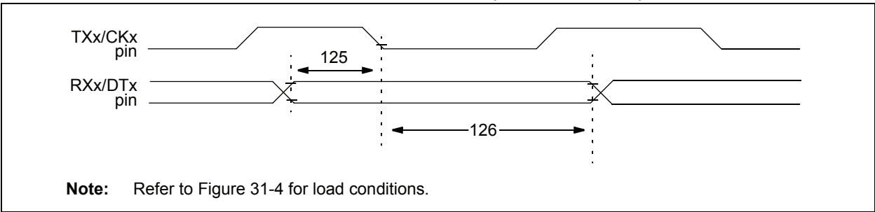
FIGURE 31-21: EUSARTx SYNCHRONOUS RECEIVE (MASTER/SLAVE) TIMING
