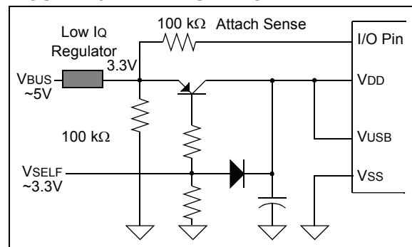
FIGURE 23-11: DUAL POWER EXAMPLE
