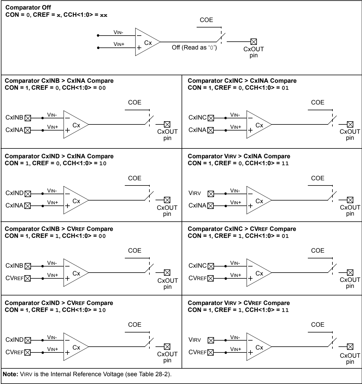
FIGURE 23-4: COMPARATOR CONFIGURATIONS
