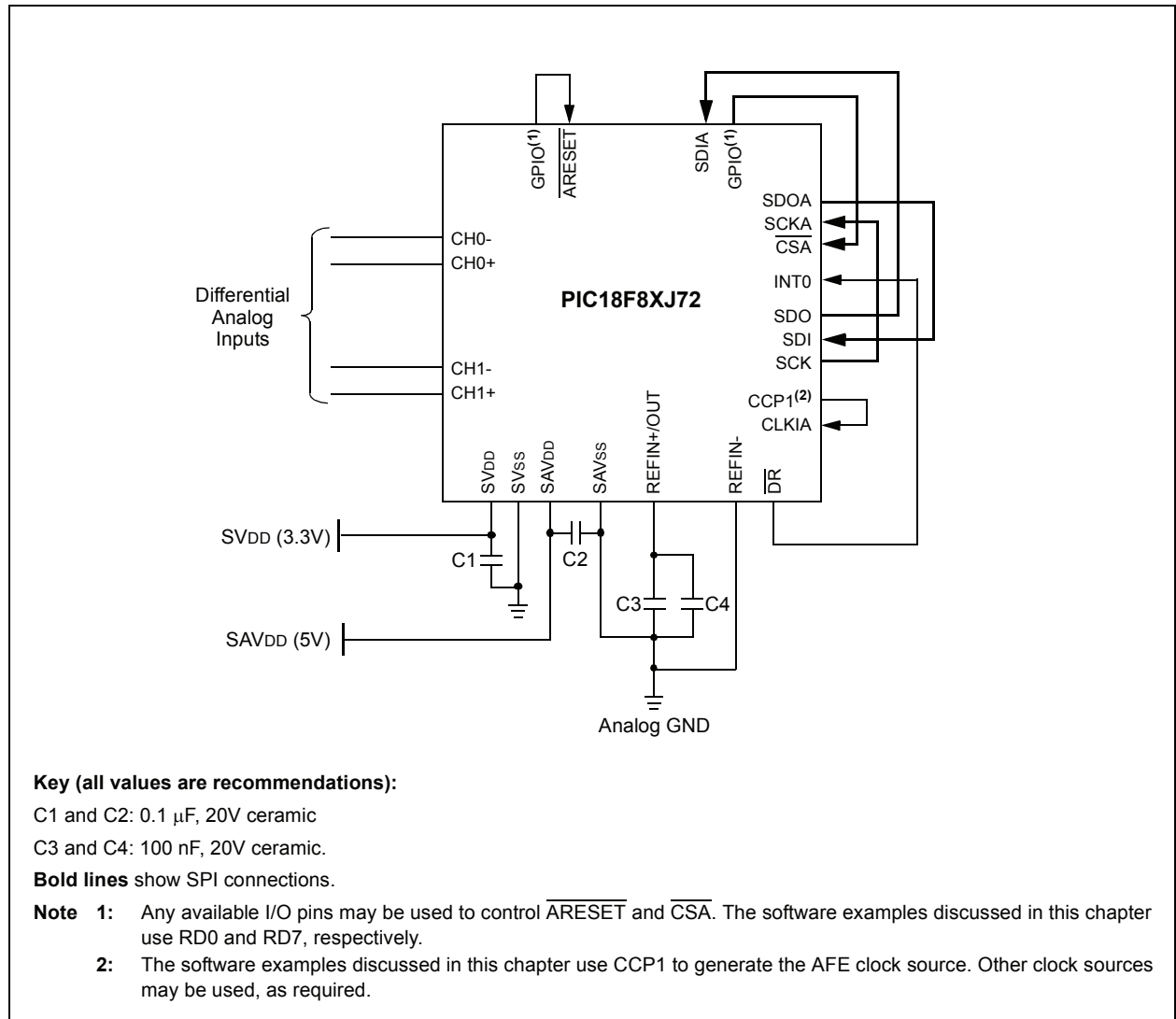
FIGURE 22-3: REQUIRED CONNECTIONS FOR AFE OPERATION
