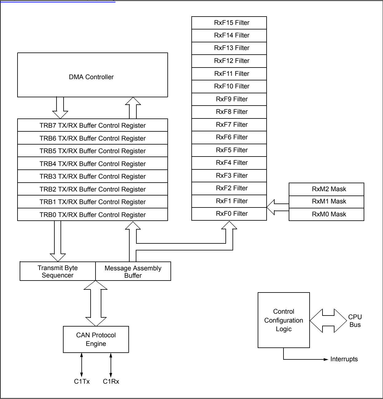
FIGURE 19-1: CAN MODULE BLOCK DIAGRAM
