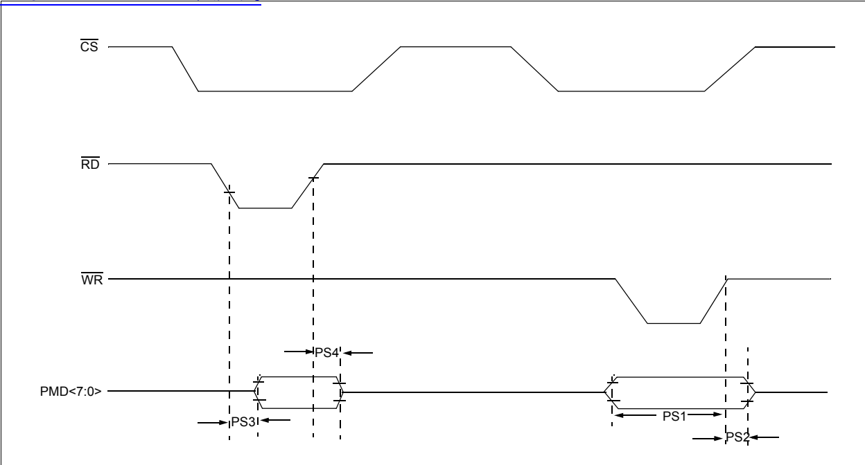
FIGURE 28-26: PARALLEL SLAVE PORT TIMING DIAGRAM
