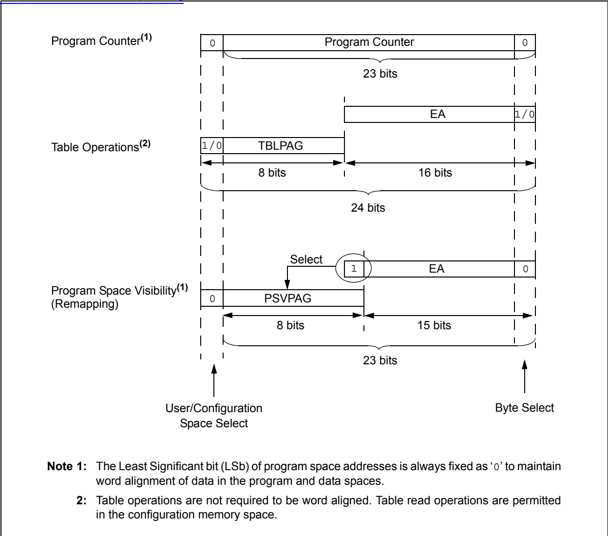
FIGURE 4-6: J64GP2 DATA ACCESS FROM PROGRAM SPACE ADDRESS GENERATION
