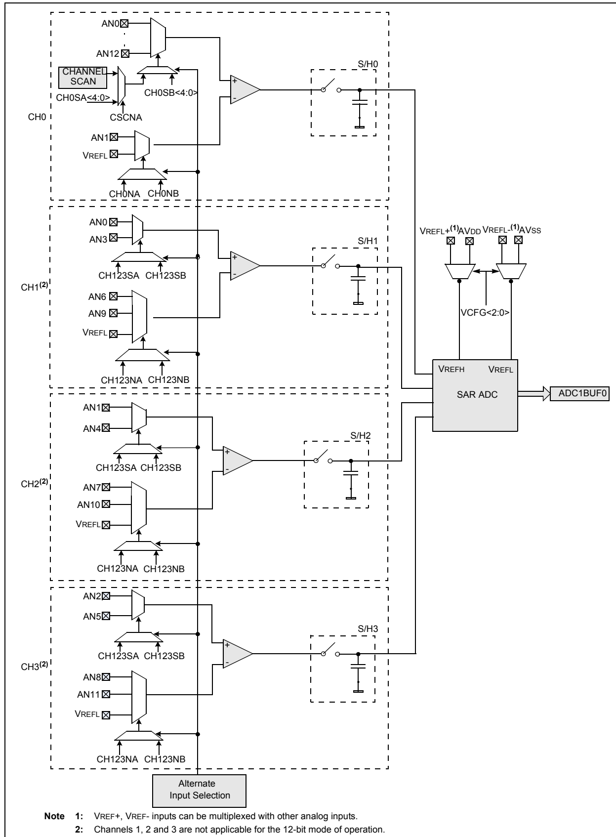
FIGURE 20-1: PIC24HJ64GPX02(X)04 ADC1 MODULE BLOCK DIAGRAM FOR PIC24HJ32GP304, PIC24HJ64GP204/504 AND PIC24HJ128GP204/504 DEVICES
