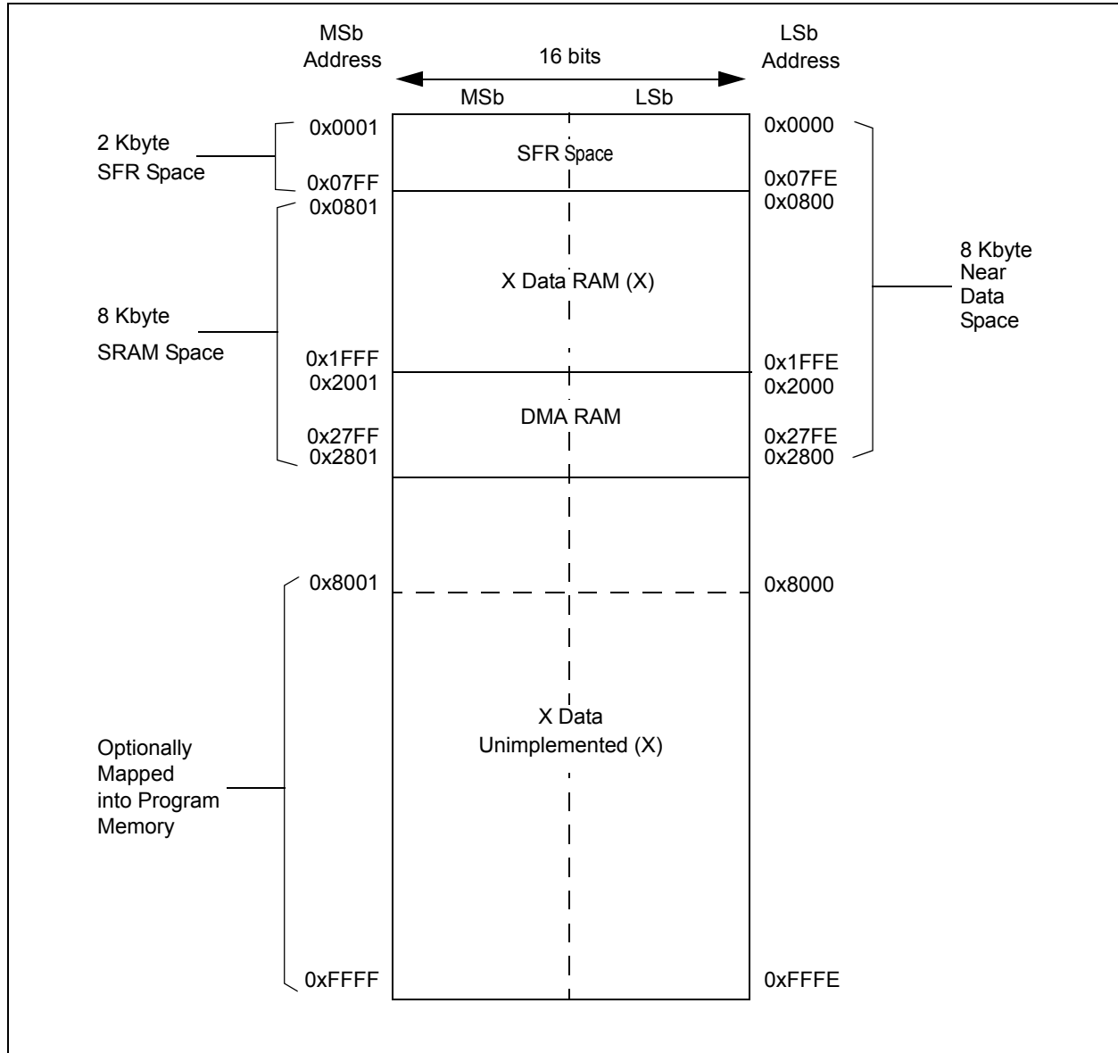
FIGURE 14-4: DATA MEMORY MAP FOR PIC24HJ128GP202/204, PIC24HJ64GP202/204, PIC24HJ128GP502/504 AND PIC24HJ64GP502/504 DEVICES WITH 8 KB RAM
