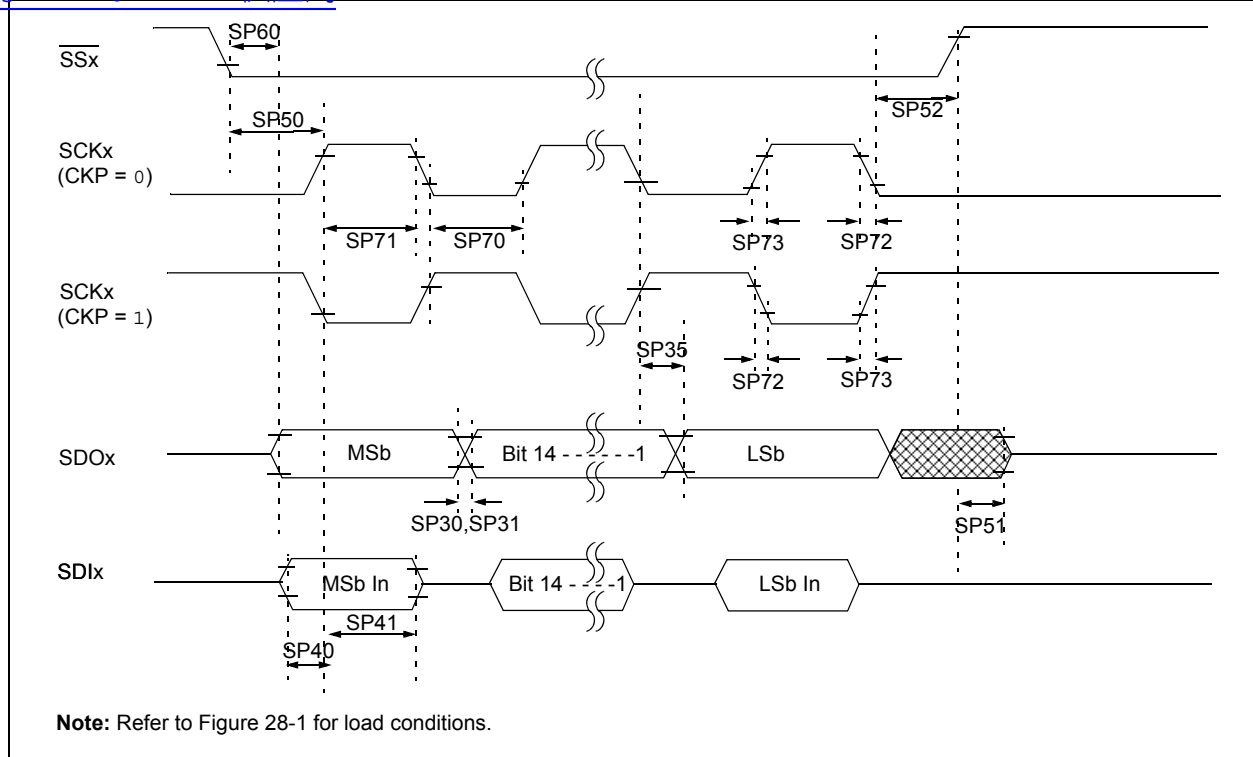
FIGURE 28-12 SPIx MODULE SLAVE MODE (CKE = 1) TIMING CHARACTERISTICS
