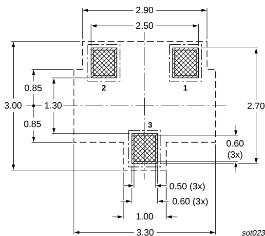
Fig 10. Reflow soldering footprint SOT23 (TO-236AB)
