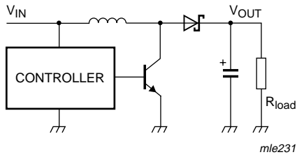
Fig 9. DC-to-DC converter
