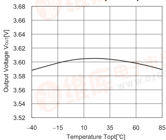
R1180x361x ( V_{IN}=4.6V )
