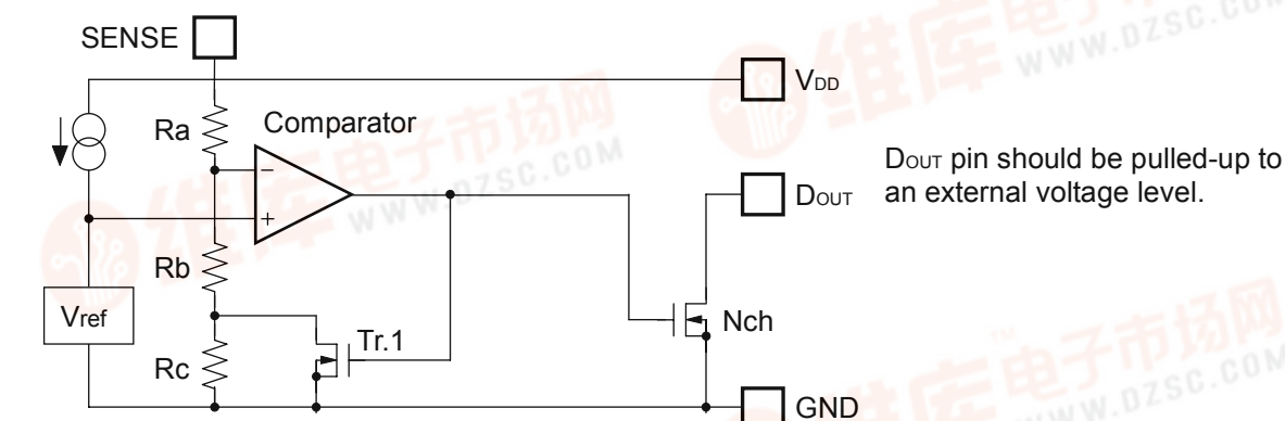
Block Diagram
