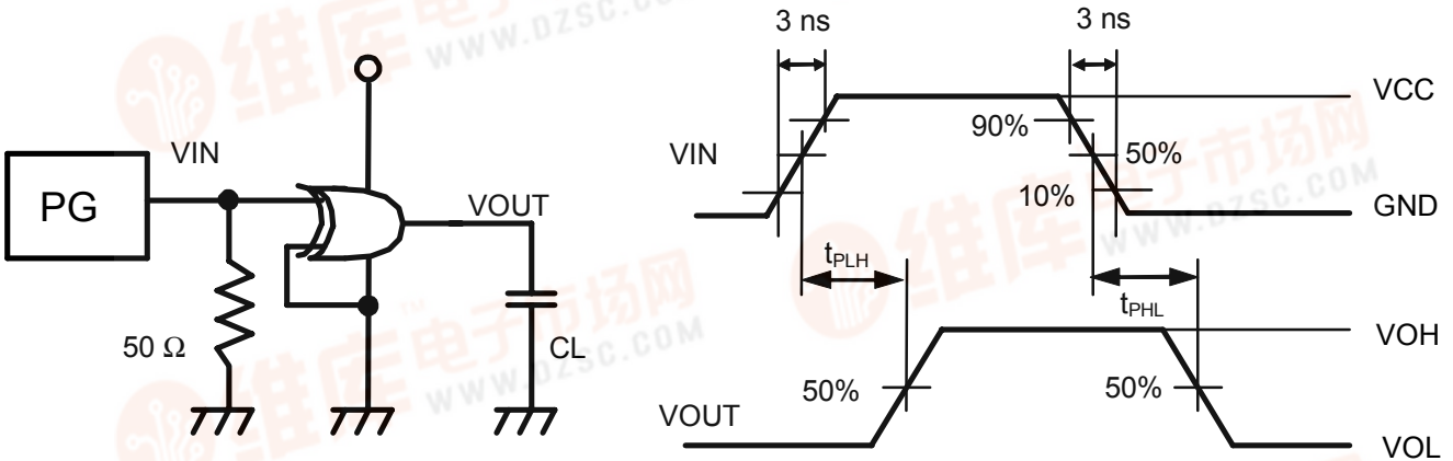
Measurement Circuit
