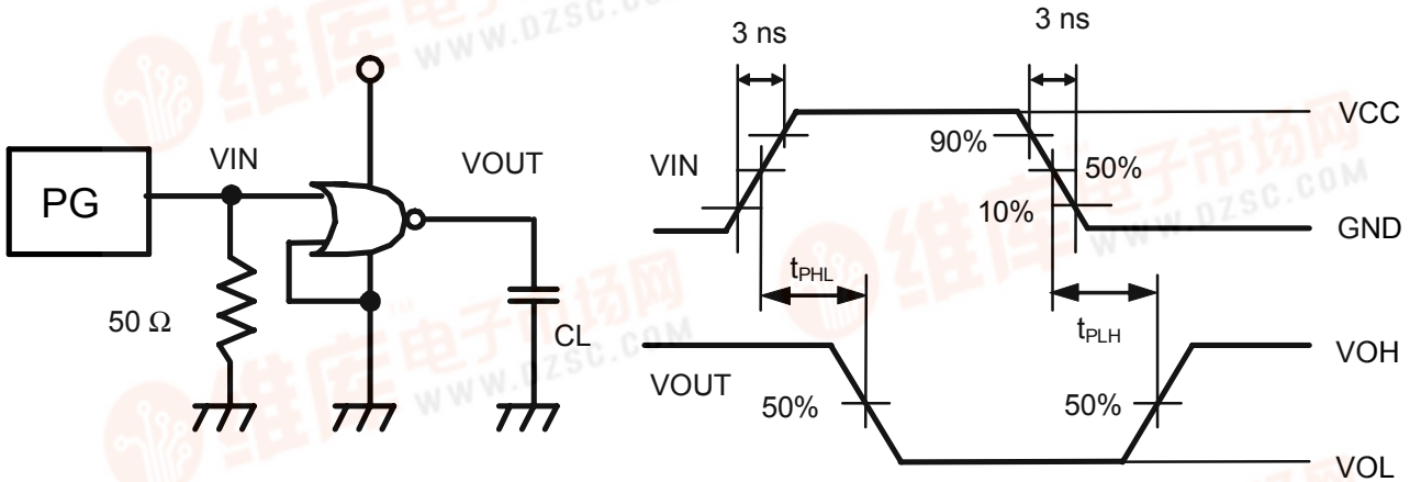
Measurement Circuit
