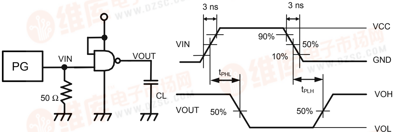
Measurement Circuit
