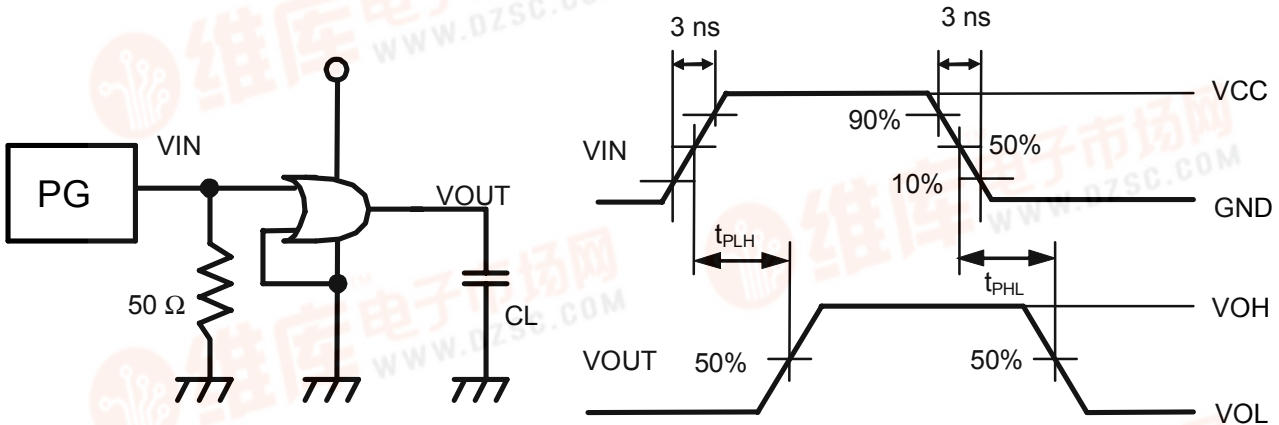
Measurement Circuit
