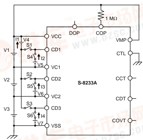
Test circuit 8
