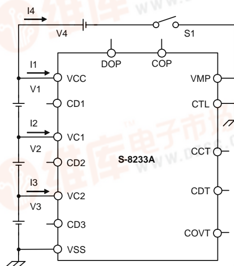
Test circuit 3
