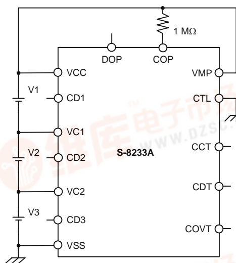
Test circuit 1
