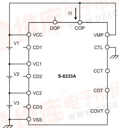
Test circuit 9
