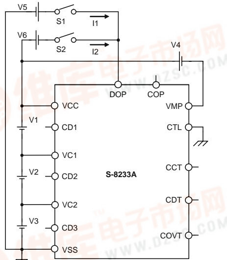
Test circuit 4
