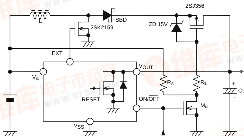
Figure 14 Circuit Example Using the 2SK2159
