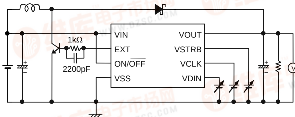
Figure 5 Measurement Circuits
