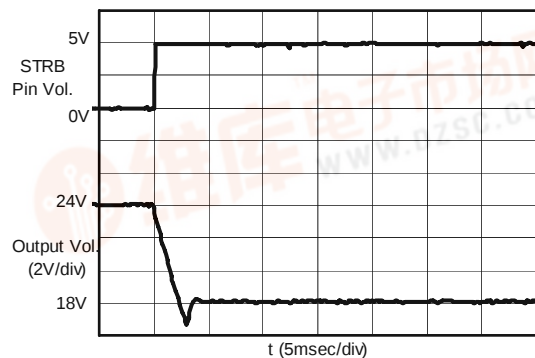
S-8331A30 ( V_{OUT}: 24V \rightarrow 18V )
