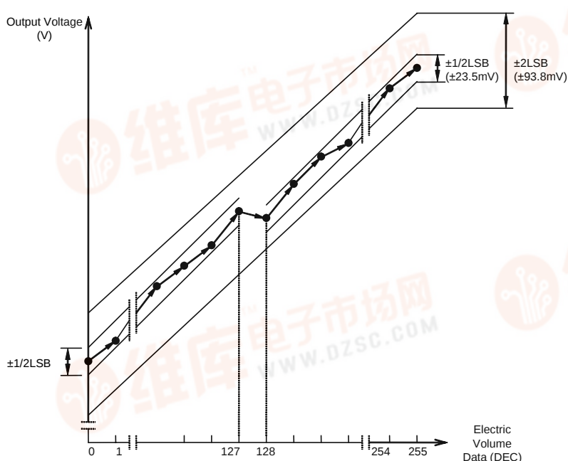
Figure 10 Linearity Accuracy
