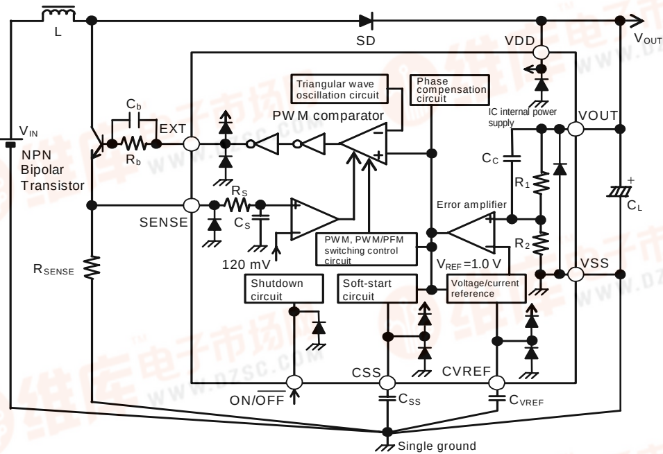
Figure 16 Output Voltage Fixed Output Type
