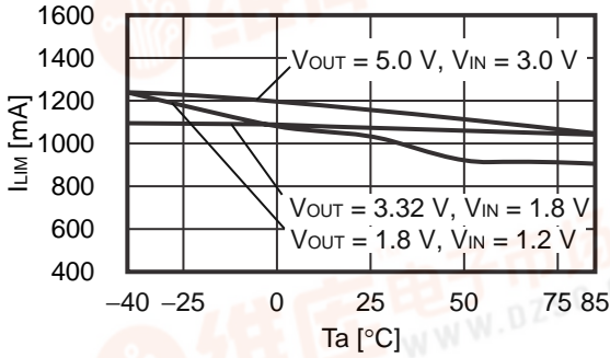
(12) Limited current (I LIM ) vs. Temperature (Ta)
