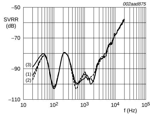
c. R_L = 2 \times 15 \mu\text{H} + 8.03 \Omega ; inputs floating (1) V_{DD} = 5.0 \text{ V} . (2) V_{DD} = 3.6 \text{ V} . (3) V_{DD} = 2.5 \text{ V} .
