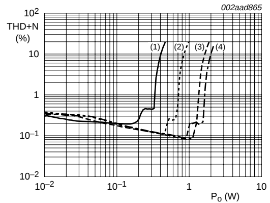
b. R_L = 2 \times 15 \mu\text{H} + 8 \Omega ; A-weighting THD+N filter
