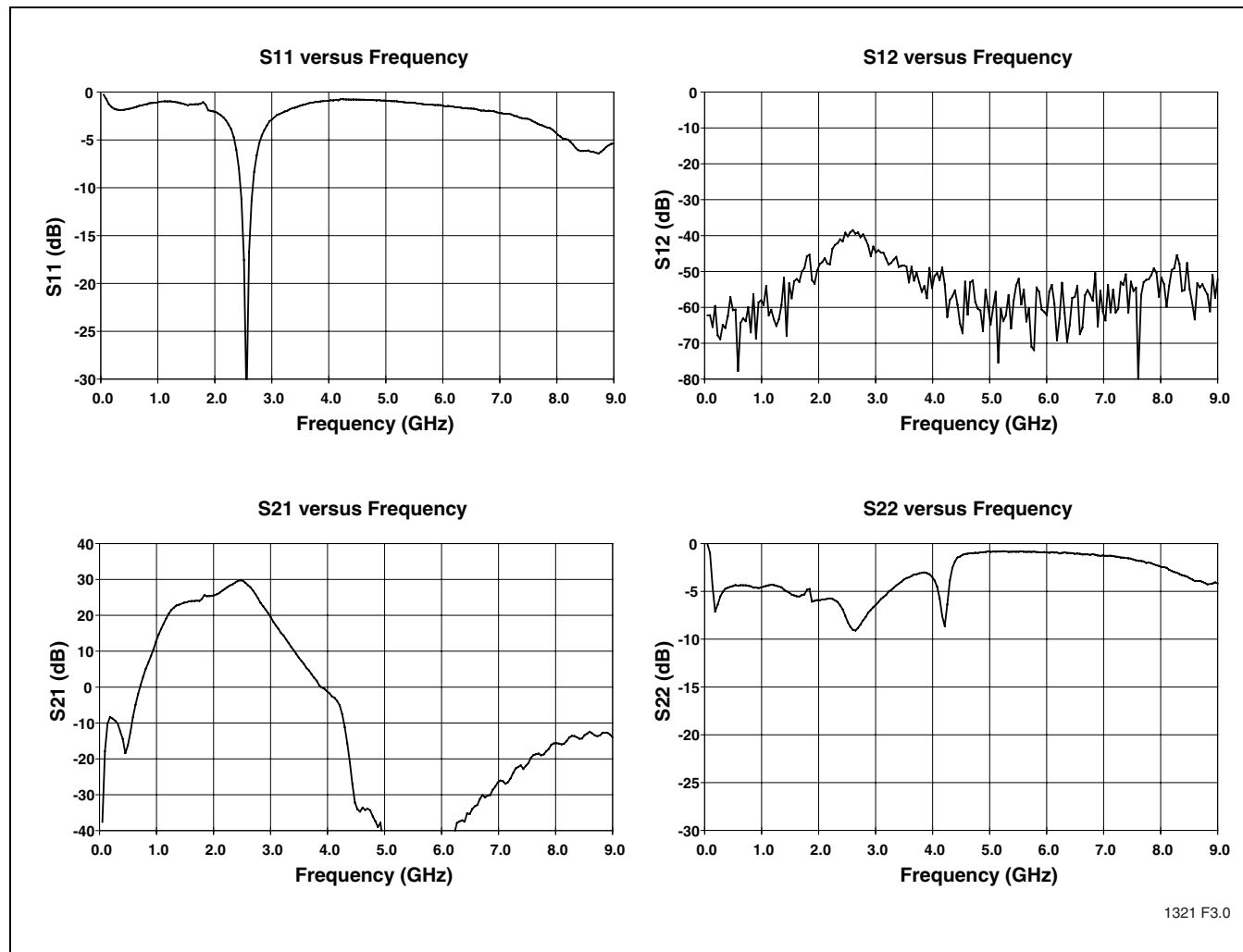
FIGURE 3: S-Parameters
