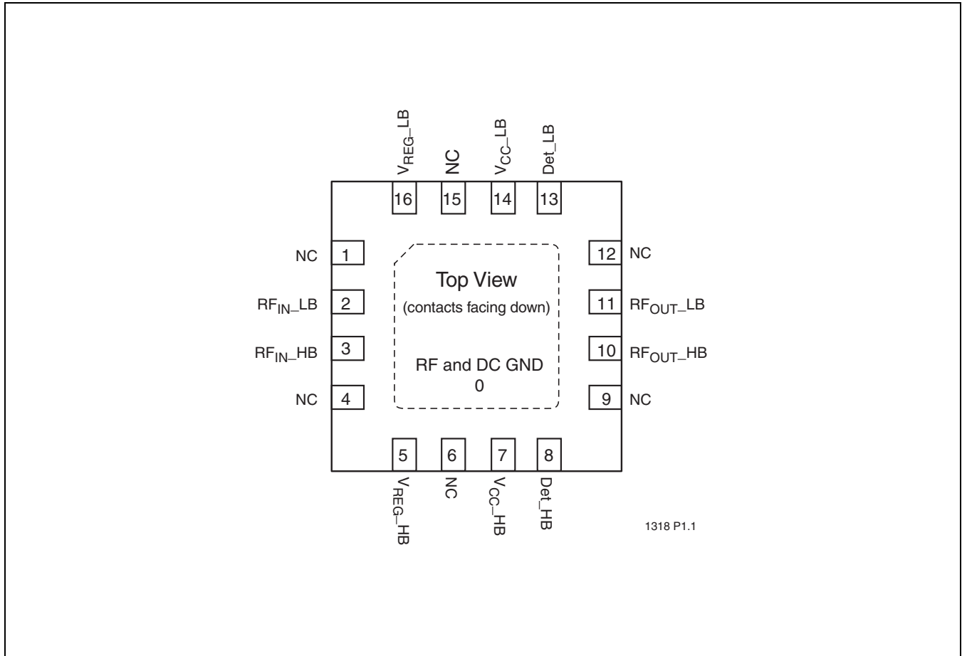
FIGURE 2: Pin Assignments for 16-contact LGA
