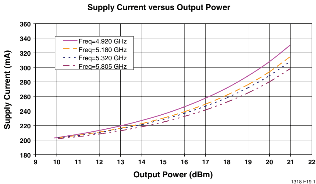
FIGURE 15: High Band Supply Current versus Output Power
