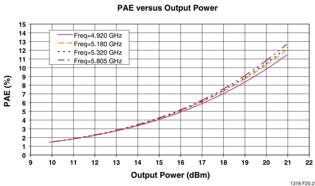
FIGURE 16: High Band PAE versus Output Power
