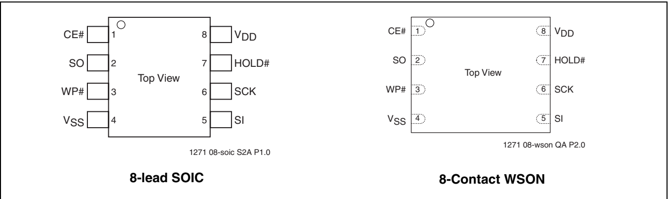
FIGURE 2: Pin Assignments
