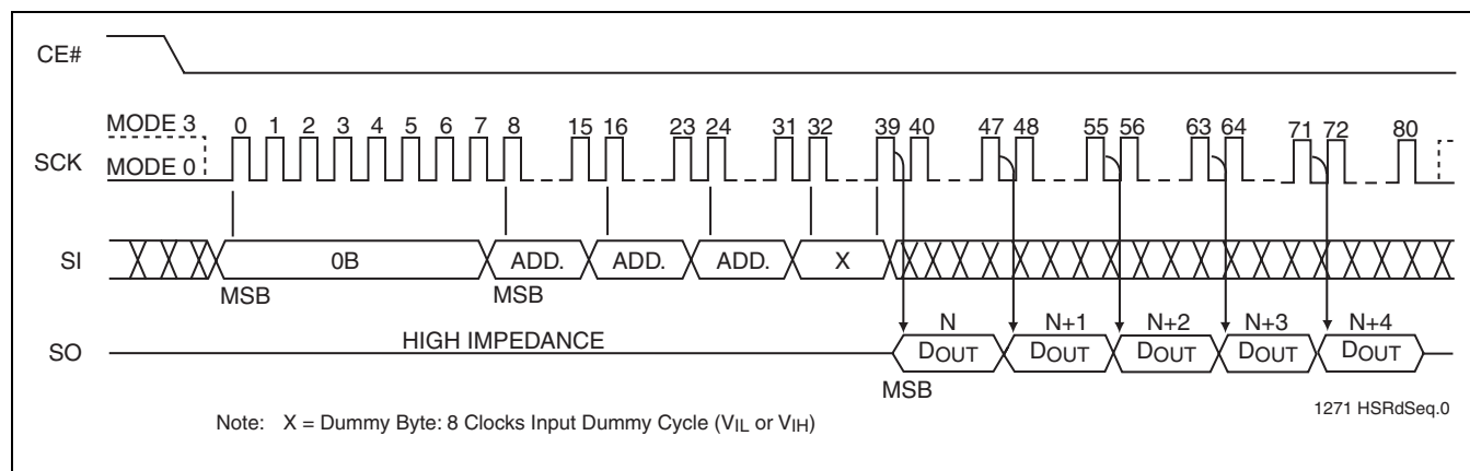
FIGURE 6: High-Speed-Read Sequence
