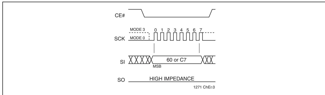
FIGURE 15: Chip-Erase Sequence
