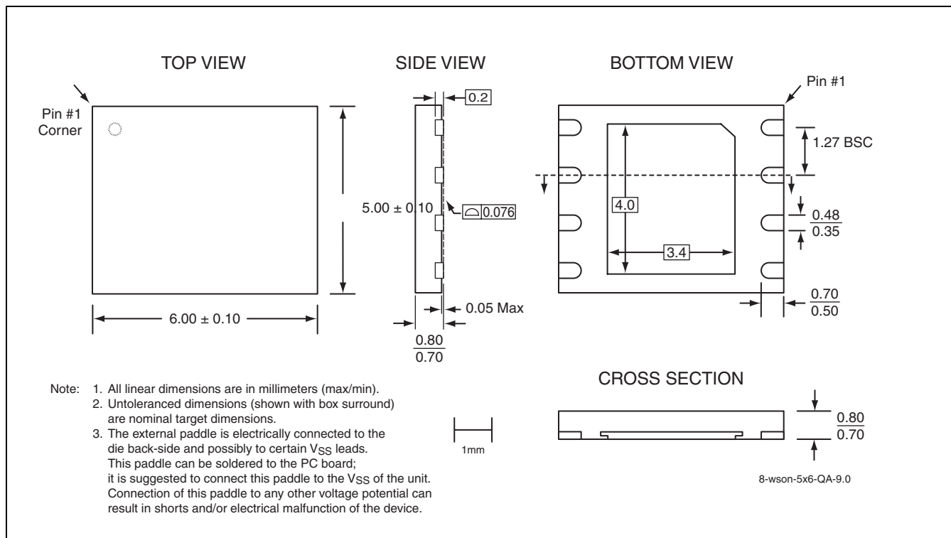
FIGURE 31: 8-Contact Very-very-thin Small Outline No-lead (WSN) SST Package Code: QA
