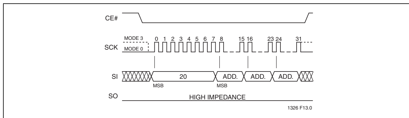
FIGURE 13: Sector-Erase Sequence
