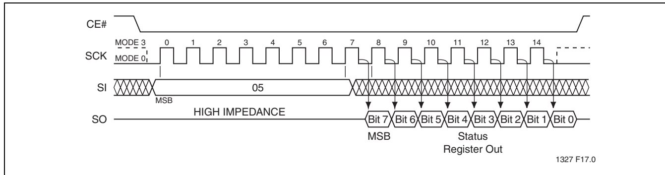
FIGURE 17: Read-Status-Register (RDSR) Sequence
