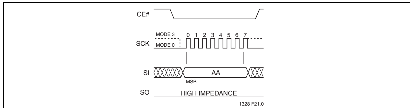
FIGURE 21: Enable-Hold Sequence
