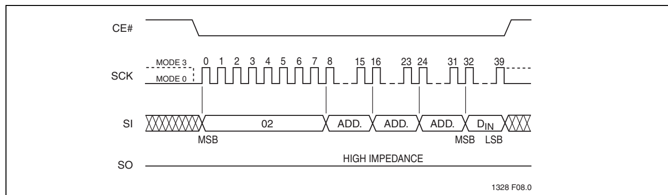
FIGURE 8: Byte-Program Sequence
