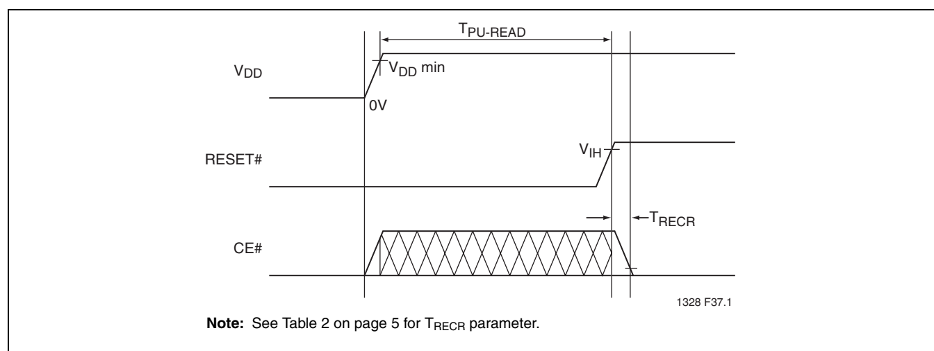
FIGURE 24: Power-Up Reset Diagram
