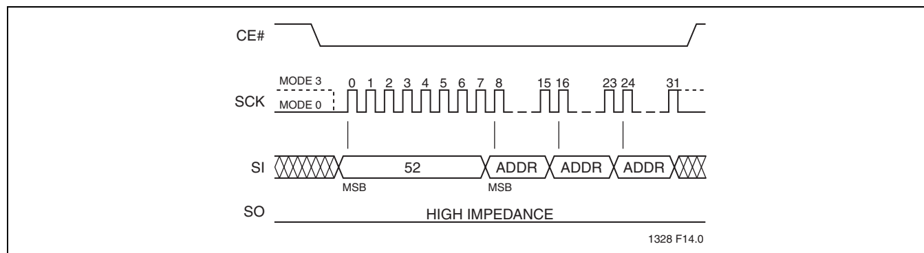
FIGURE 14: 32-KByte Block-Erase Sequence
