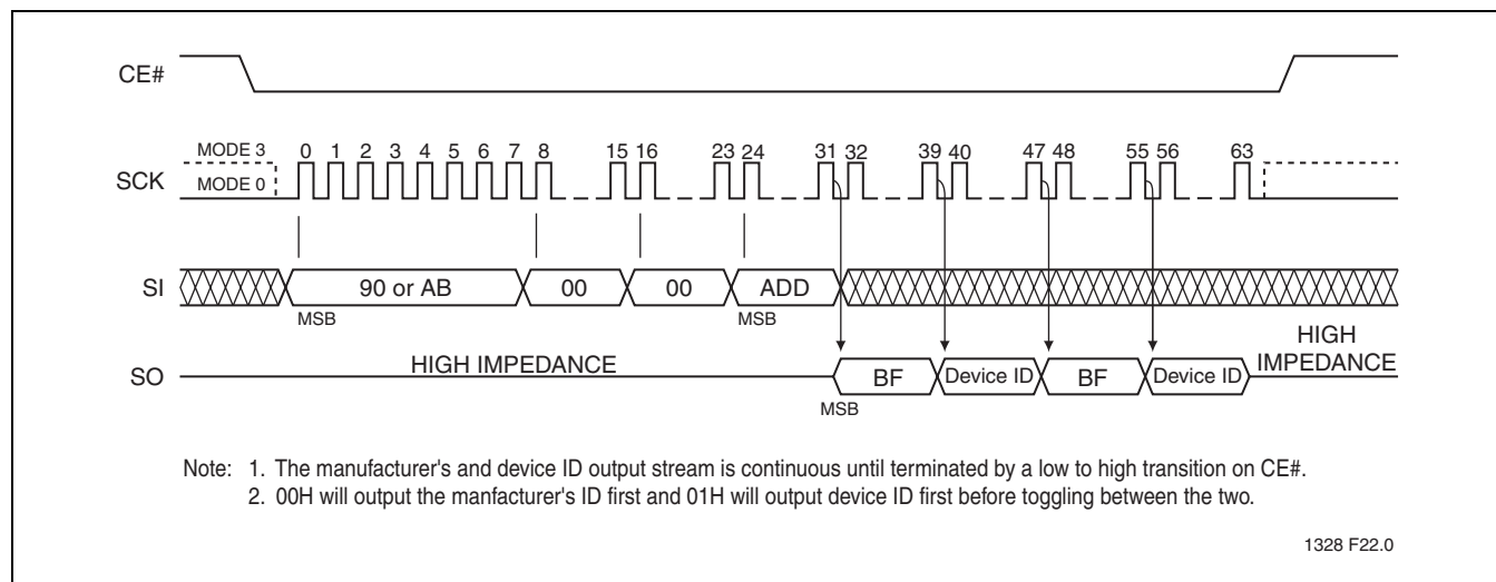
FIGURE 22: Read-ID Sequence
