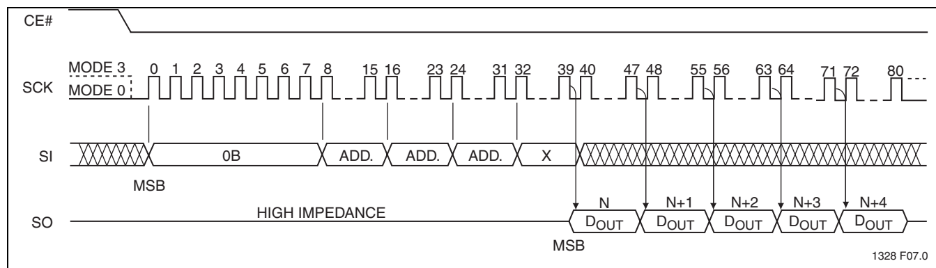
FIGURE 7: High-Speed-Read Sequence
