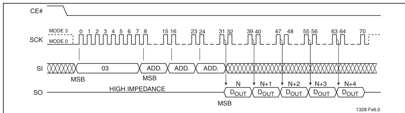
FIGURE 6: Read Sequence
