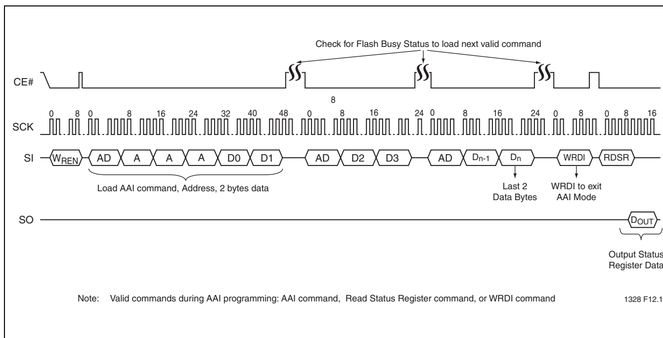
FIGURE 12: Auto Address Increment (AAI) Word Program Sequence with Software End-of-Write Detection
