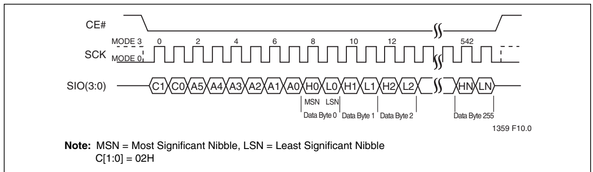
Figure 18: Page-Program Sequence
