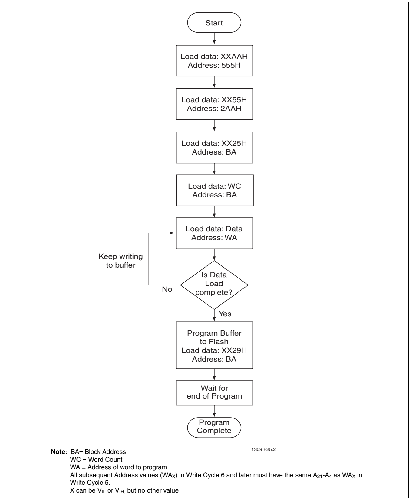
FIGURE 25: Write-Buffer Programming
