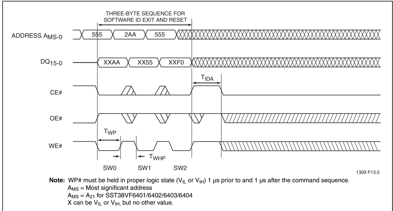
FIGURE 18: Software ID Exit/CFI Exit
