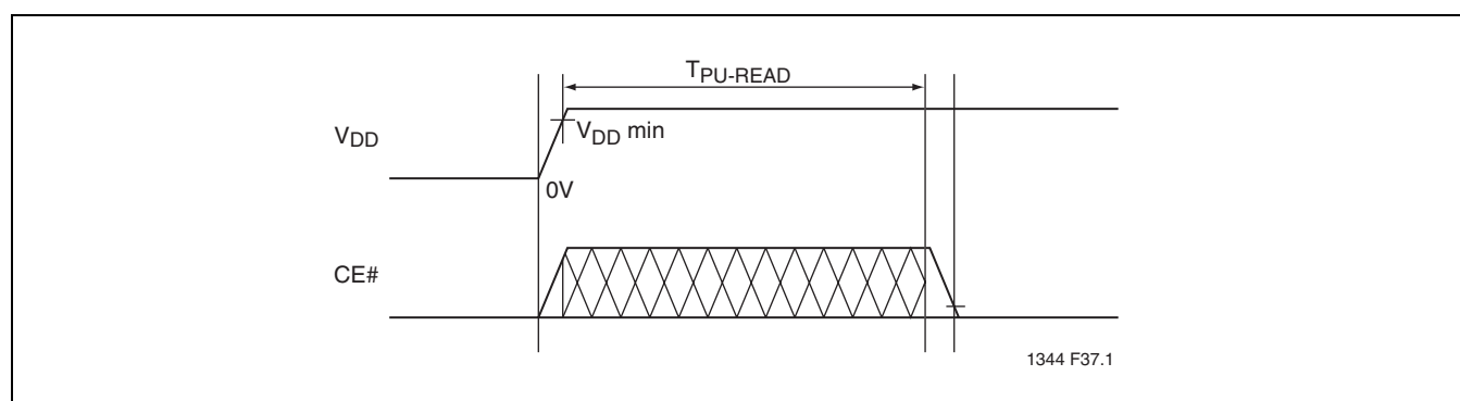
FIGURE 4: Power-Up Reset Diagram
