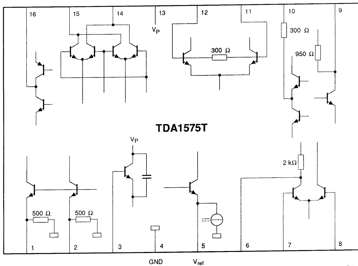
Fig.10 Internal circuits.
