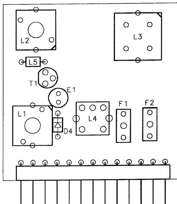
Component Side
