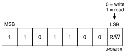
Fig.7 Address byte.
