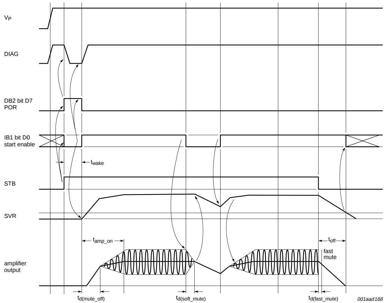
Fig 3. Start-up and shut-down timing in I 2 C-bus mode
