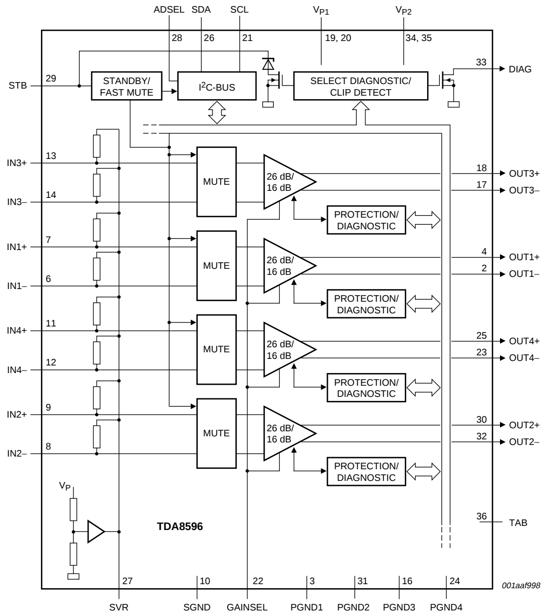
Fig 1. Block diagram
