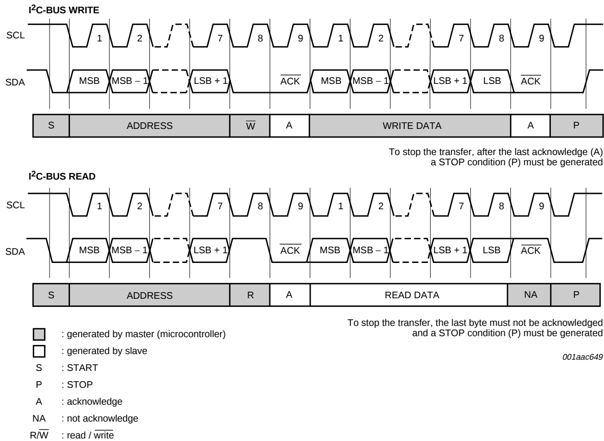
Fig 16. I 2 C-bus read and write modes
