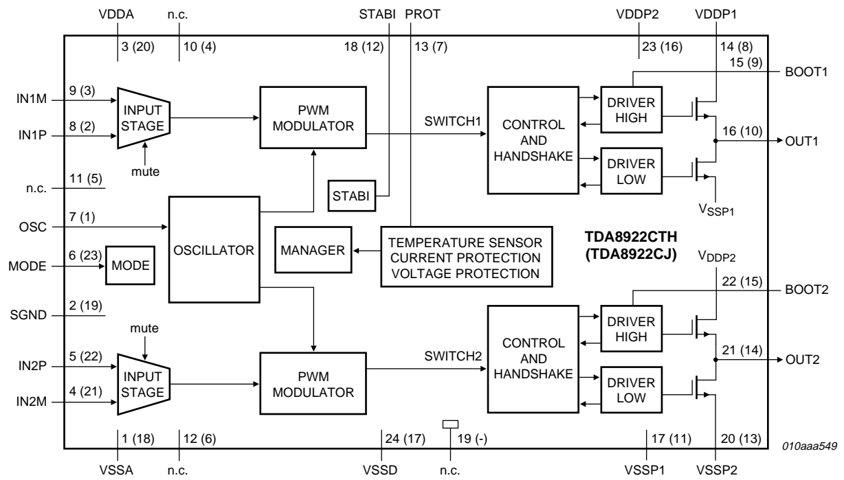
Fig 1. Block diagram
