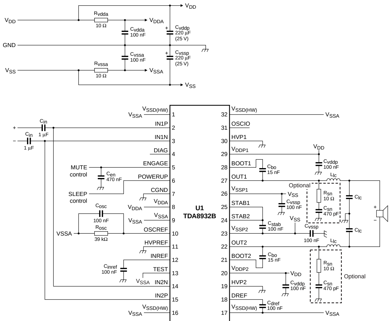
Fig 35. Typical simplified application diagram for 1 x BTL (symmetrical supply)
