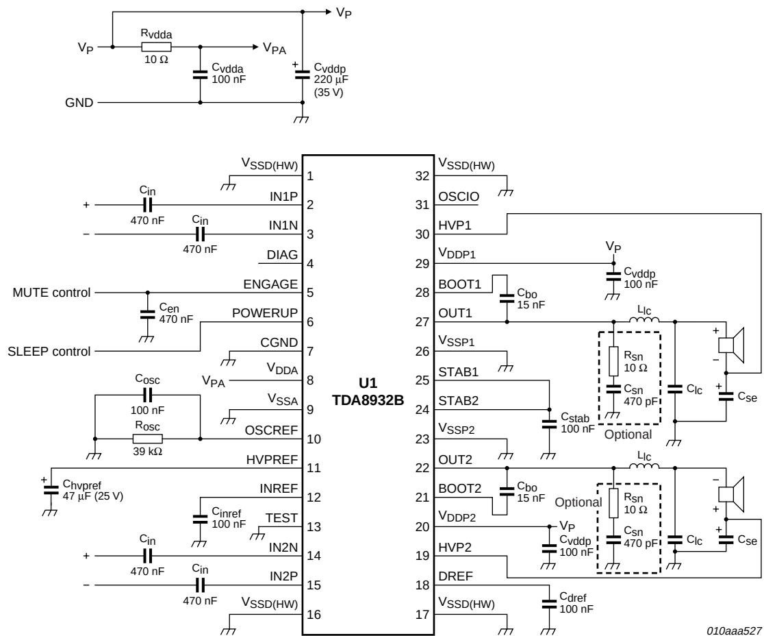
Fig 32. Typical simplified application diagram for 2 × SE (asymmetrical supply)
