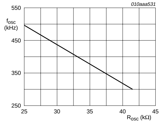
Fig 4. Oscillation frequency as a function of R_{osc}
