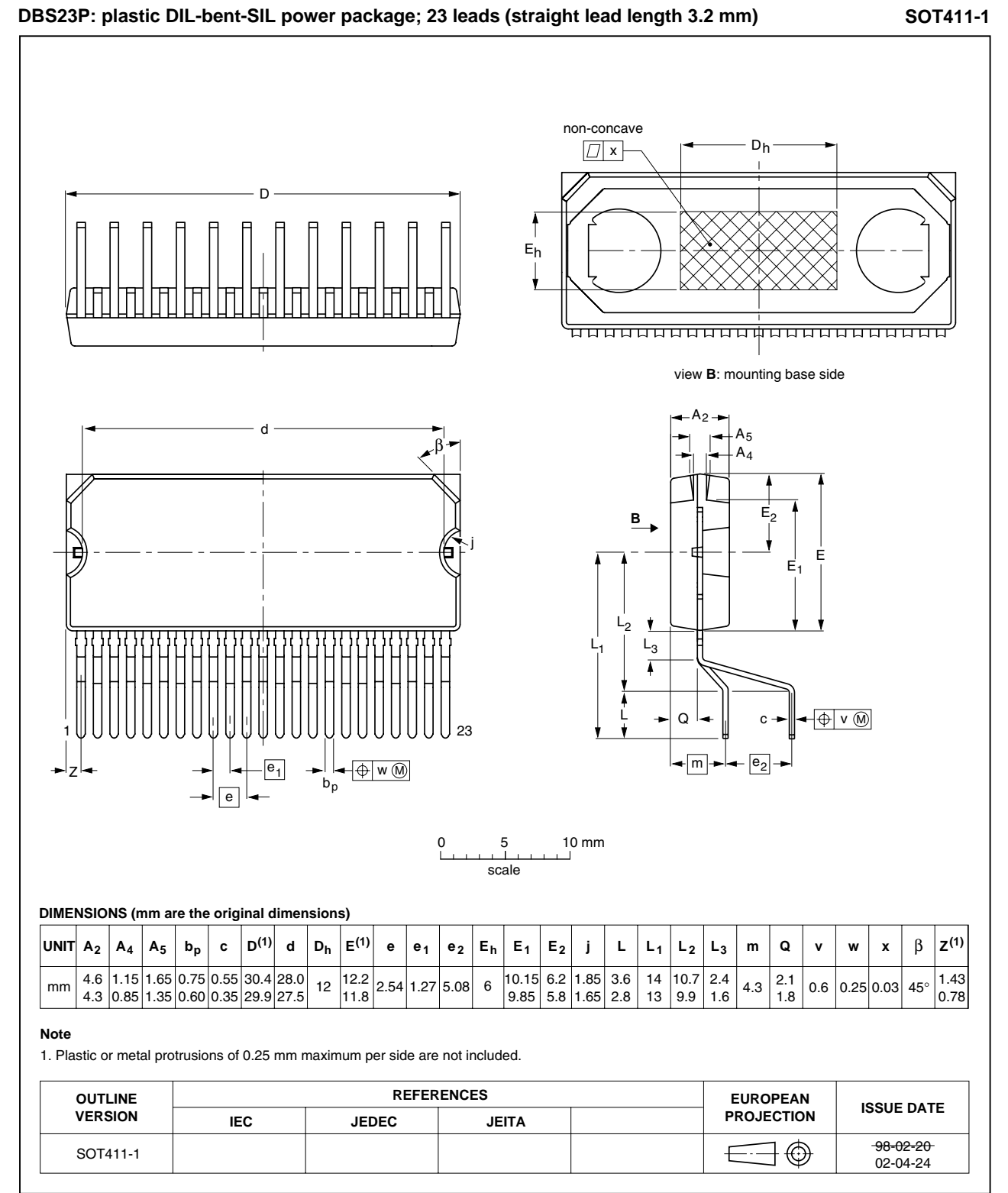
Fig 34. Package outline SOT411-1 (DBS23P)
