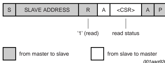
Fig 4. Host reads TDA9950 Status Register - after setting address pointer
