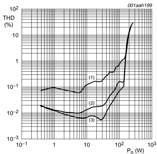
Fig 12. Total harmonic distortion as a function of output power, SE application
