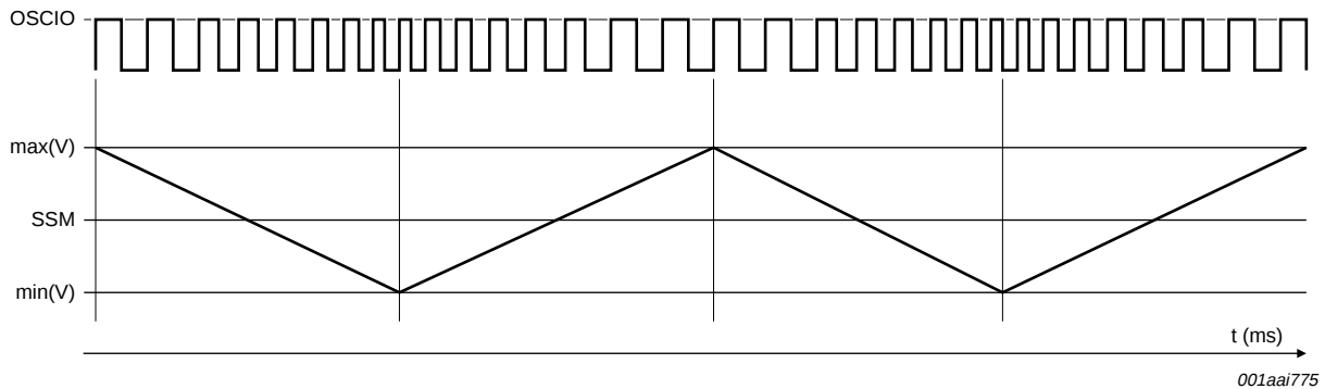
Fig 7. Spread spectrum operation in Master mode
