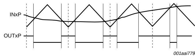
a. Bridge half 1.
