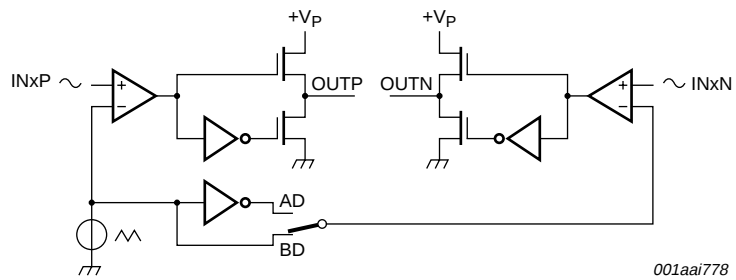
Fig 9. AD/BD modulation switching circuit
