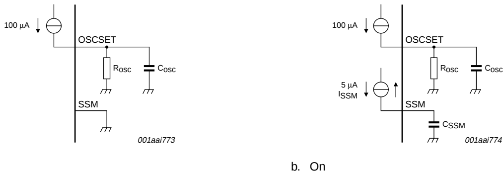
Fig 6. Spread spectrum mode
