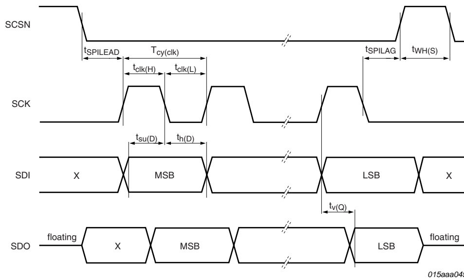
Fig 19. SPI timing diagram
