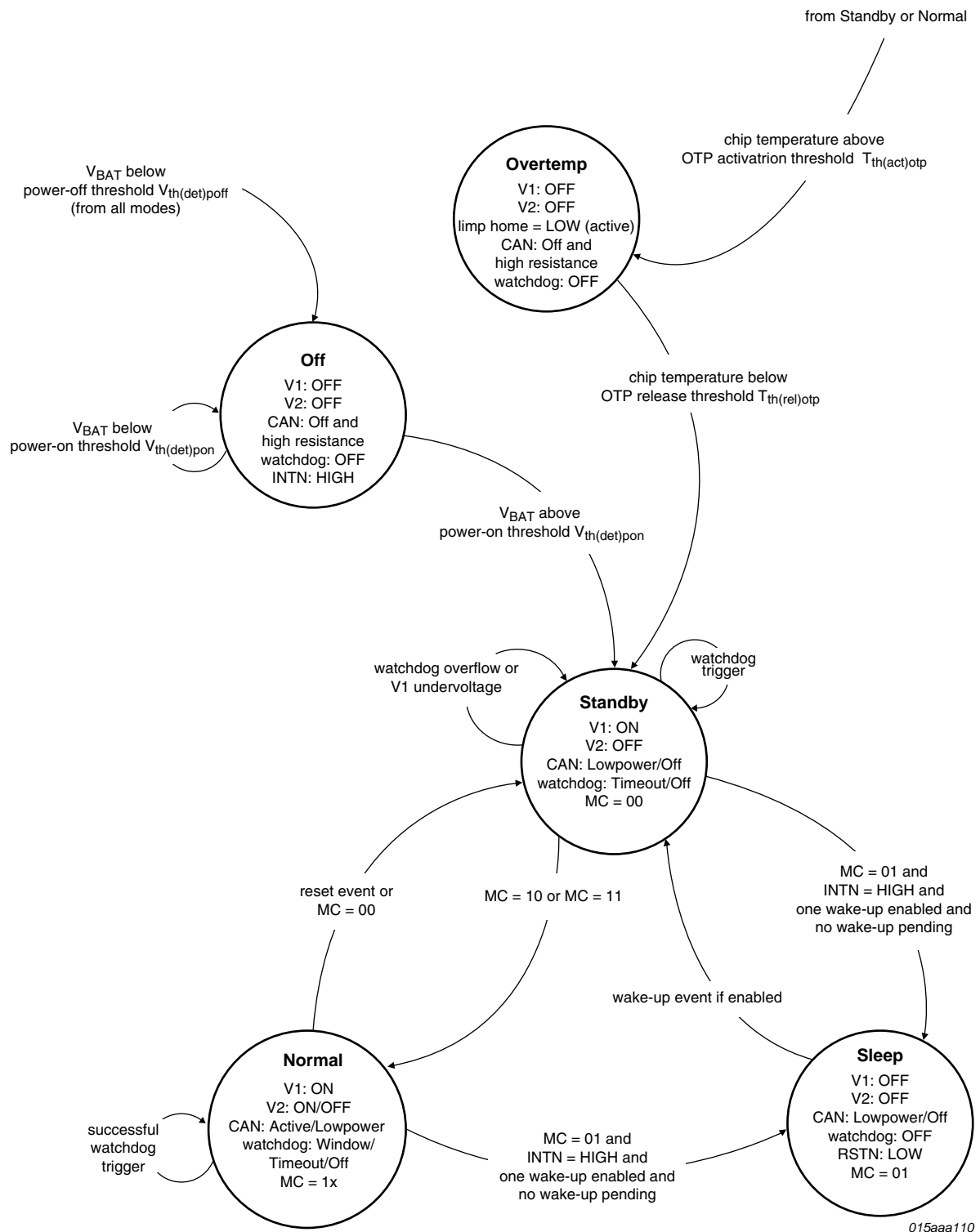
Fig 3. UJA1076 system controller
