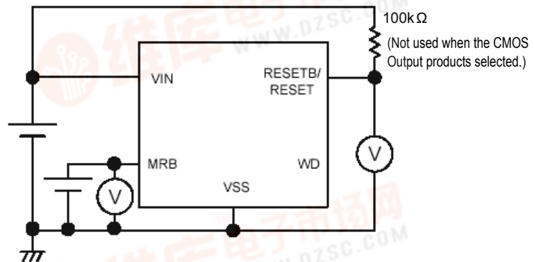
Circuit 9
