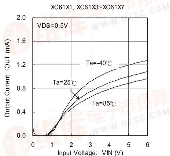
(7) P-ch Driver Output Current vs. Input Voltage 2
