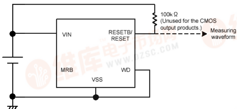
Circuit 6
