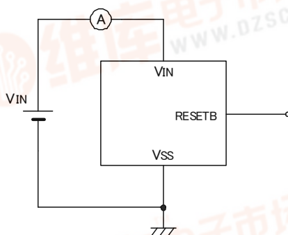
● Circuit ④
