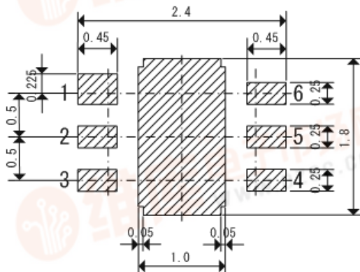
USP-6B Recommended Pattern Layout
