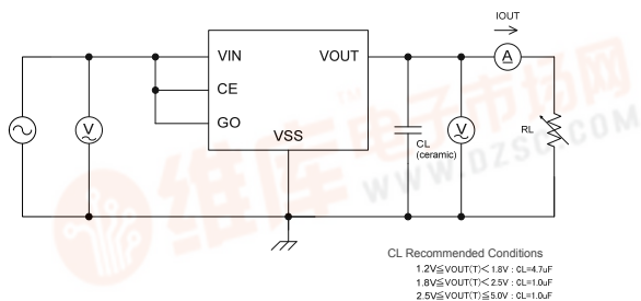
Circuit 4 CE/GO, High & Low Level Voltage
