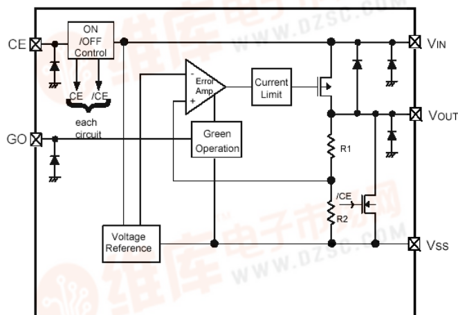
XC6207B Series
