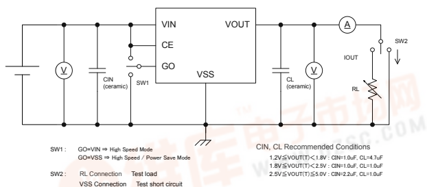
Circuit 2 Supply Current, Standby Current
