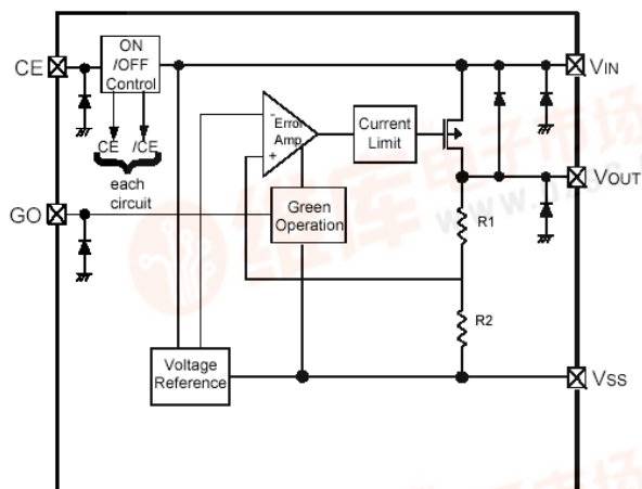
XC6207A Series
