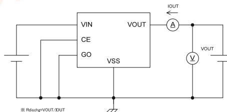
Circuit 7 CL Auto-Discharge Resistance Current
