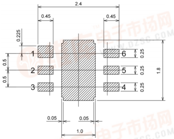
● USP-6B Reference Pattern Layout
