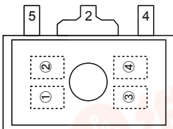
SOT-89-5 (TOP VIEW)
