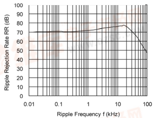
XC6219/11x252 VIN=2.8V, DC+1Vp-pAC IOU=50mA, CL=1uF (ceramic)
