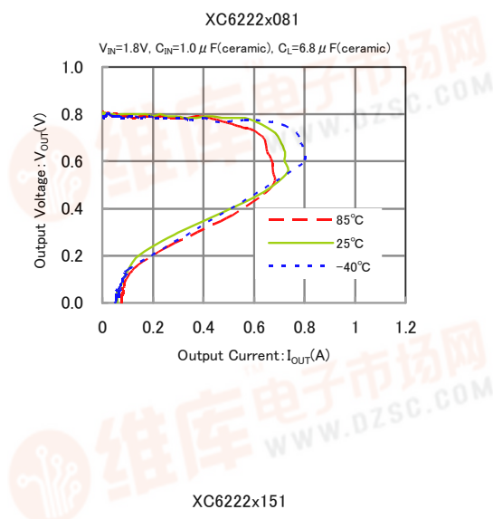
(1) Output Voltage vs. Output Current
