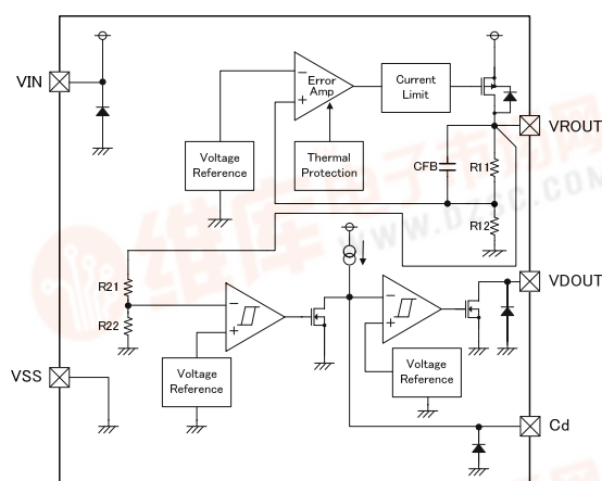
XC6408 D Type
