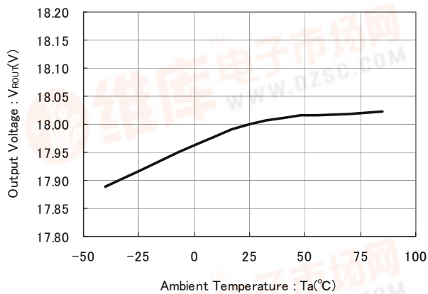
XC6408D/E ( V_{ROUT}=18.0V , I_{ROUT}=20mA )
