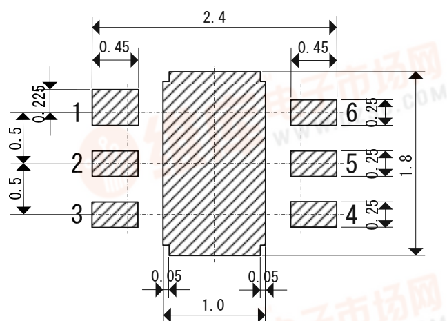
● USP-6C Reference Pattern Layout
