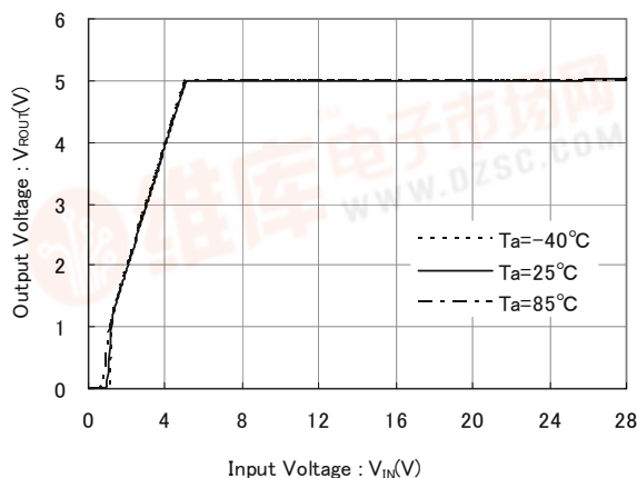
XC6408D/E ( V_{ROUT}=5.0V , I_{ROUT}=5mA )
