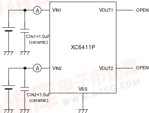
Circuit ②
