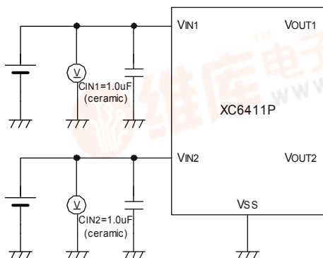
Circuit ①
