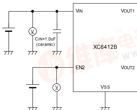
Circuit ①
