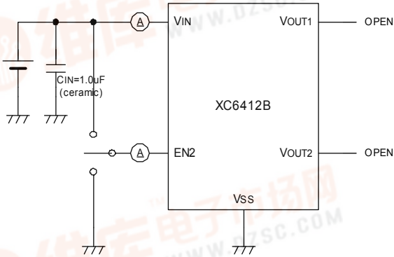
Circuit ②
